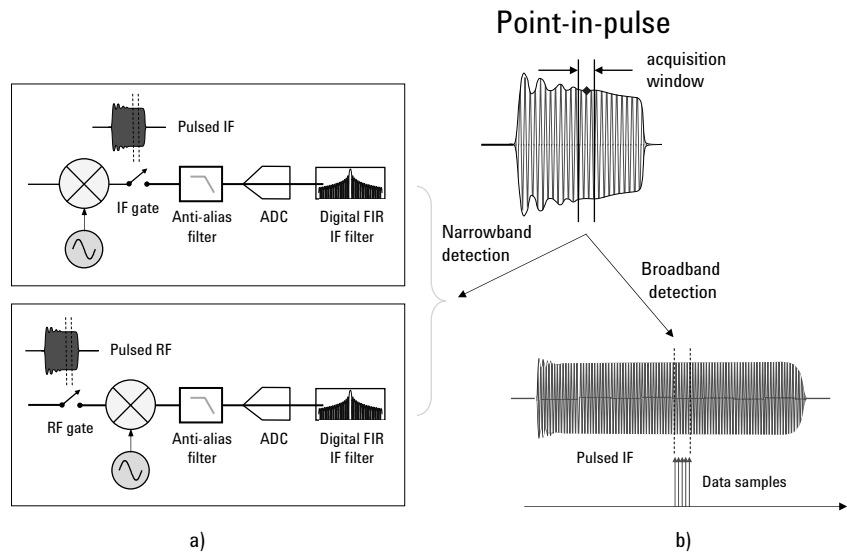
Figure 4. a) Narrowband detection uses hardware switches (gates) in the RF or IF path to define the acquisition window. b) Broadband detection uses the sampling period to define the acquisition window.
