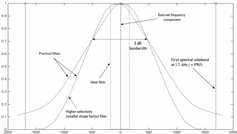
Figure 23. A zoomed-in view of the example pulse spectrum showing ideal and practical filter responses
