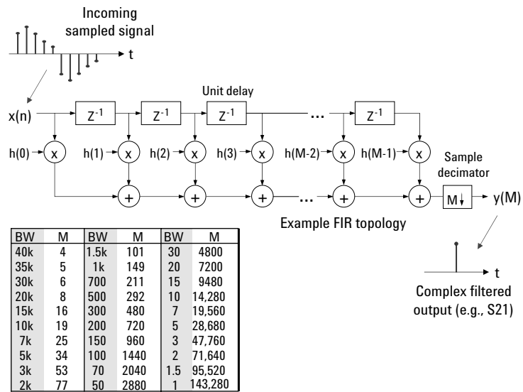
Figure 25. Finite impulse response (FIR) filter basics
