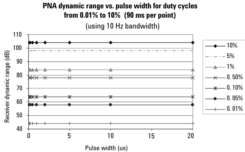
Figure 48. PNA dynamic range versus pulse width for various duty cycles
